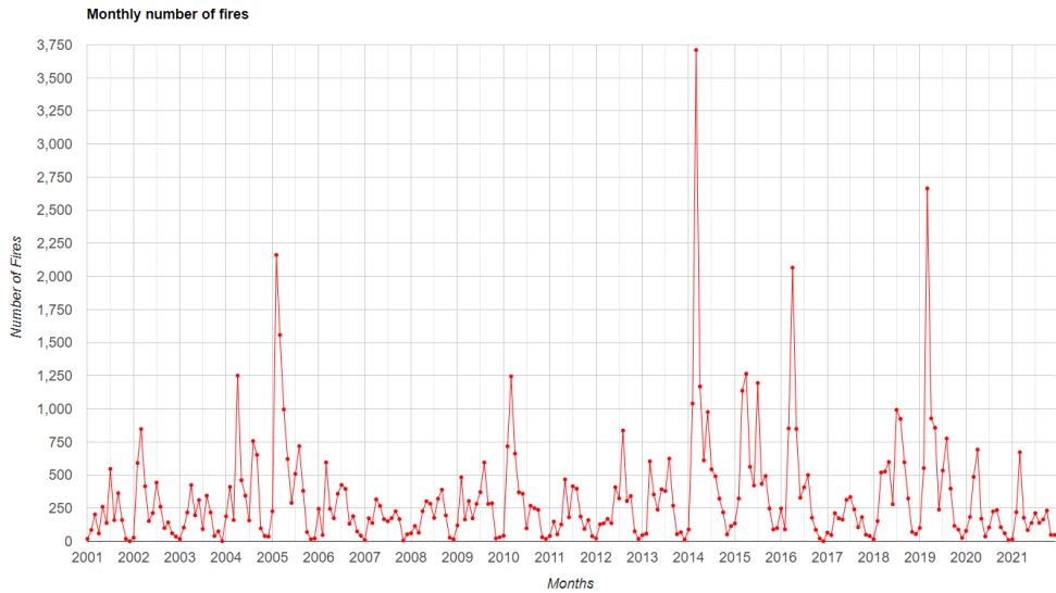
Fig. 4: Total number of hotspots detected monthly arranged in chronological order from 1st January 2001 to 31st December 2021
